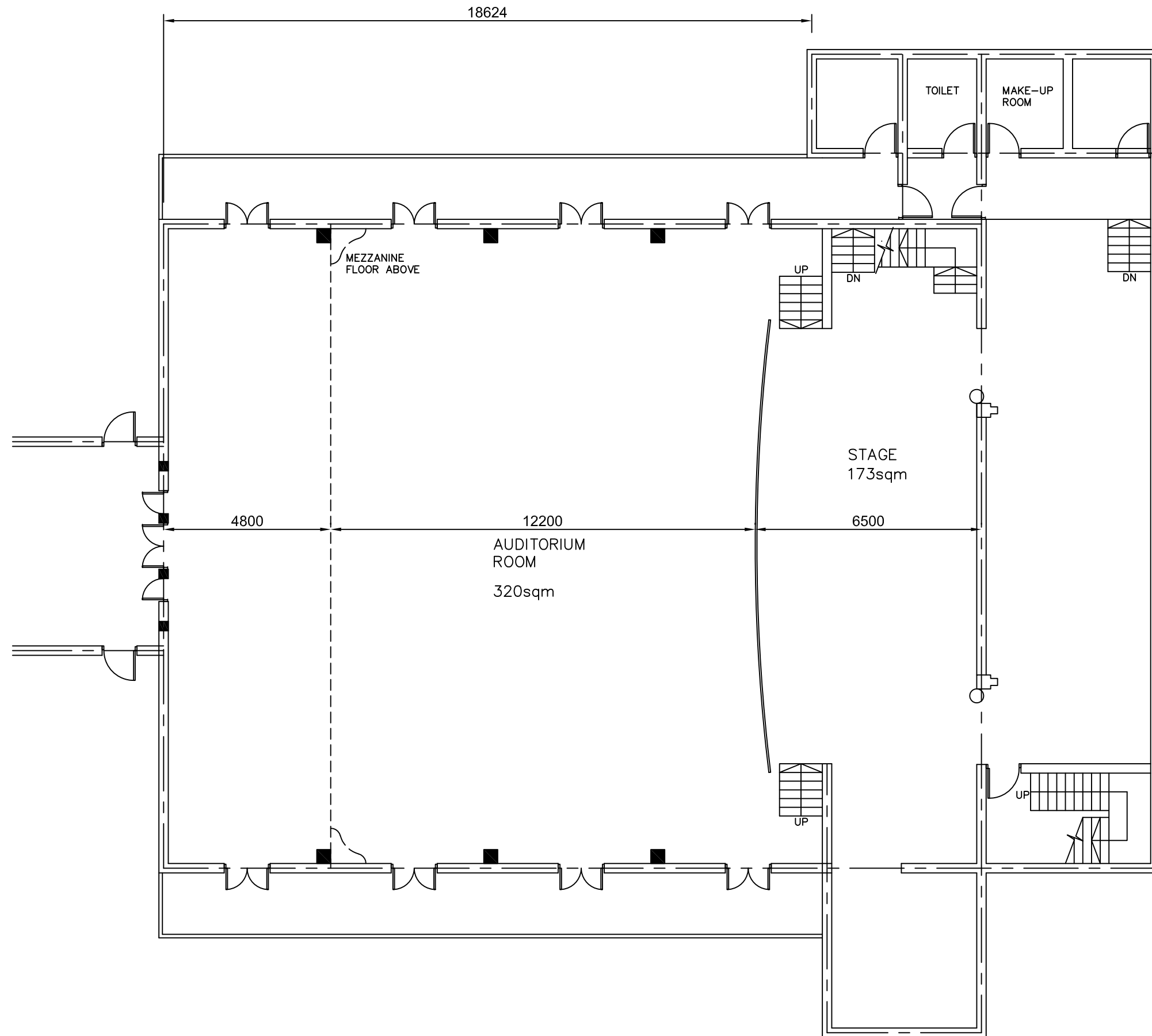
2ND STOREY PLAN SCCCI BUILDING SCALE 1:125
